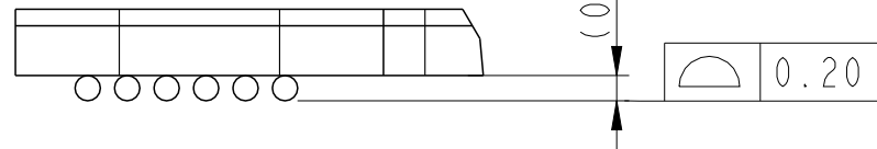
DETAIL F SCALE 5:1
