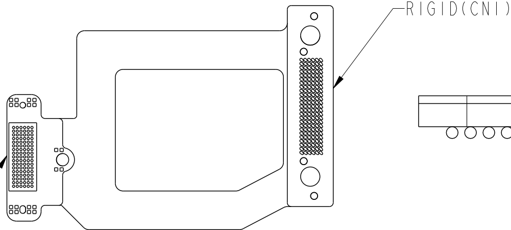
DETAIL F SCALE 5:1
