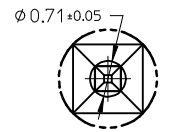
DETAIL 7
