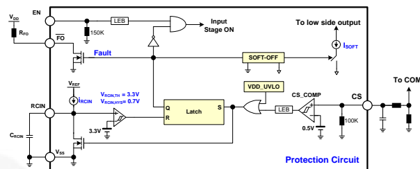
Figure 42. Over-Current Protection
