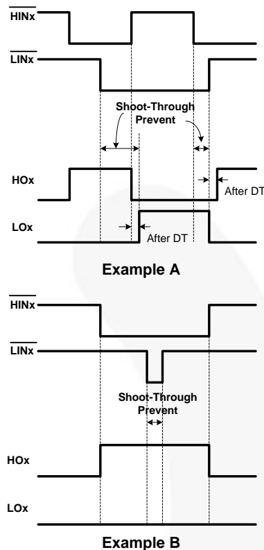
Figure 39. Shoot-Through Protection
