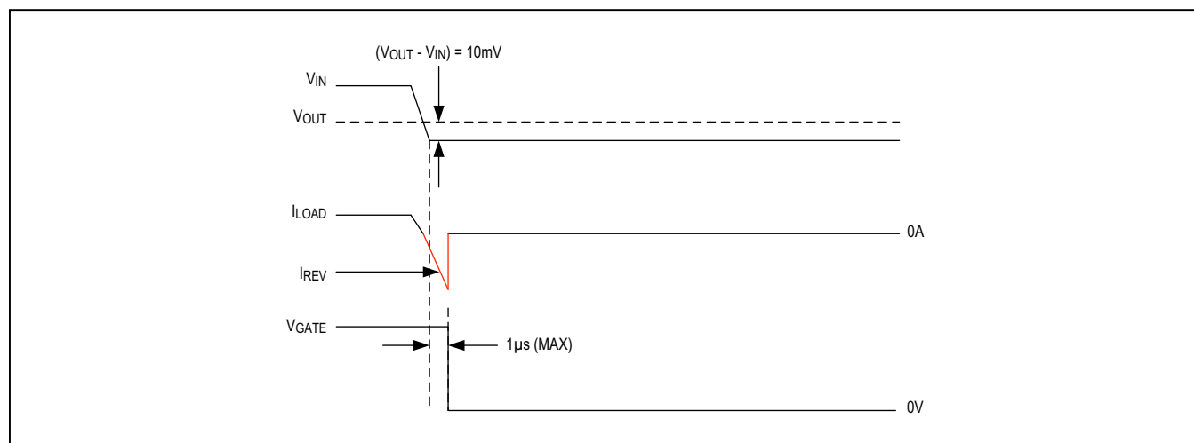
Figure 3. Reverse-Voltage Fault
