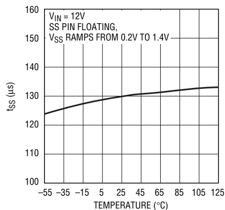
t_{SS} vs Temperature
