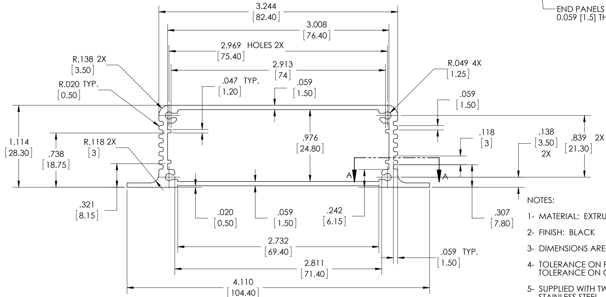
EXTRUSION PROFILE
