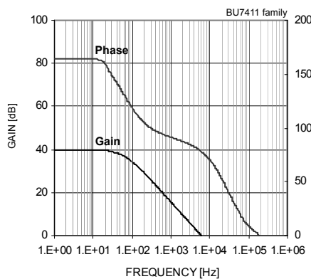
Fig.69 Gain – Frequency
