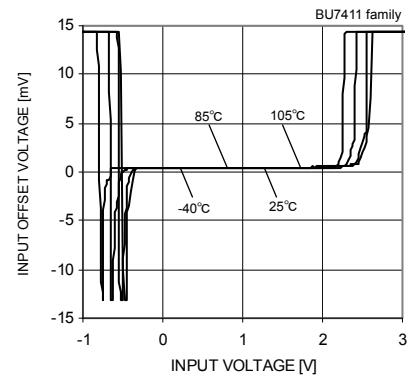
Fig.61 Input Offset Voltage – Input Voltage (VDD=3[V])
