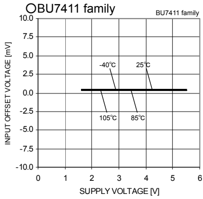
Fig.59 Input Offset Voltage – Supply Voltage (Vicm=VDD-1[V], VOUT=1.5[V])
