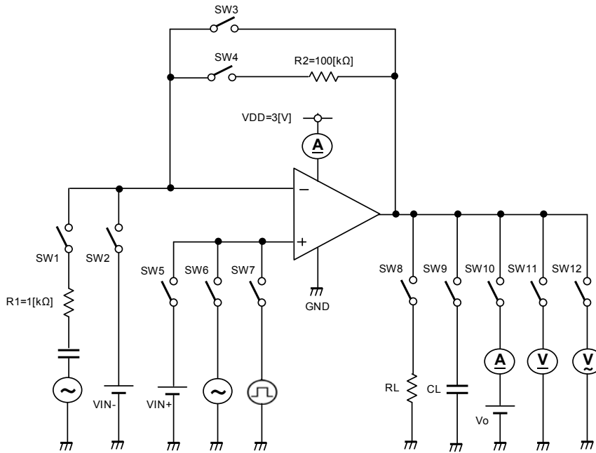
Fig.95 Test circuit2
