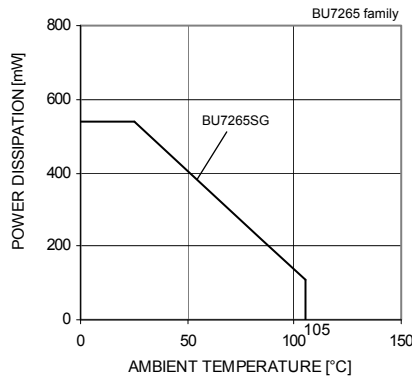
Fig.2 Derating curve
