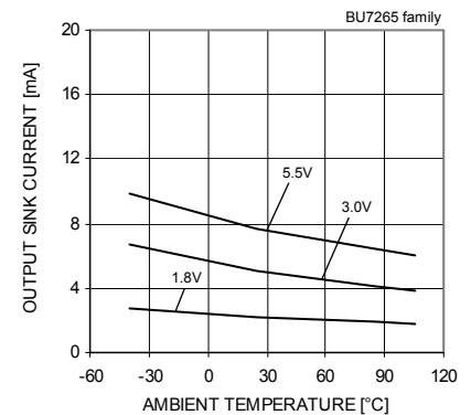
Fig.12 Output Sink Current - Ambient Temperature (VOUT=VSS+0.4[V])
