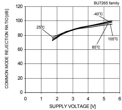
Fig. 18 Common Mode Rejection Ratio – Supply Voltage
