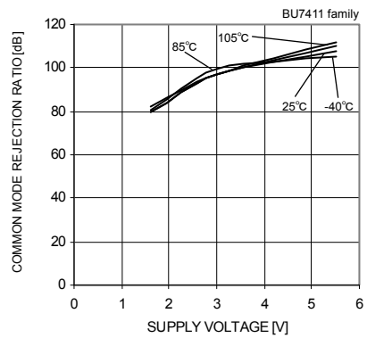
Fig.64 Common Mode Rejection Ratio – Supply Voltage
