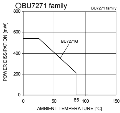
Fig.24 Derating curve
