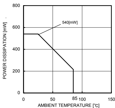
(c) BU7265G BU7271G BU7411G BU7421G
