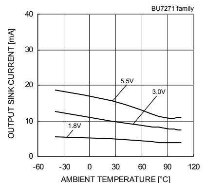
Fig.35 Output Sink Current - Ambient Temperature (VOUT=VSS+0.4[V])
