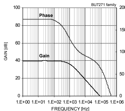
Fig. 46 Gain – Frequency
