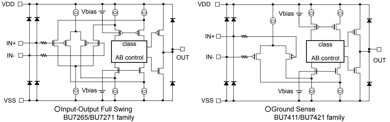
Fig.93 Schematic Diagram
