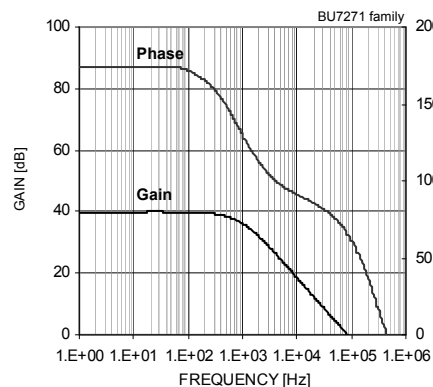
Fig. 46 Gain – Frequency
