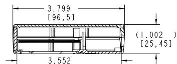
PANEL TO REAR SURFACE SECTION B-B
