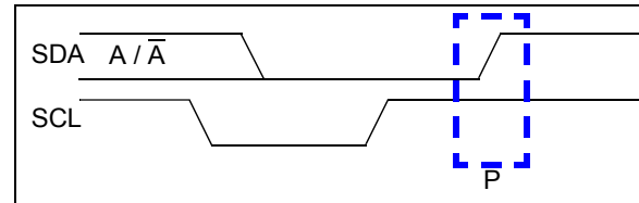
FIGURE 2-6: STOP CONDITION RECEIVE OR TRANSMIT MODE
