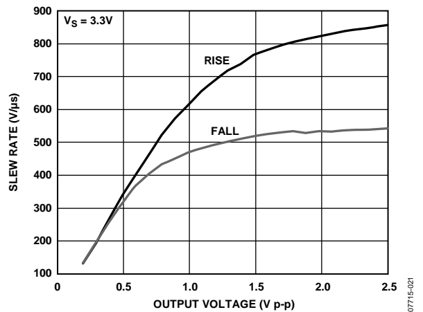
Figure 21. Slew Rate vs. Output Voltage
