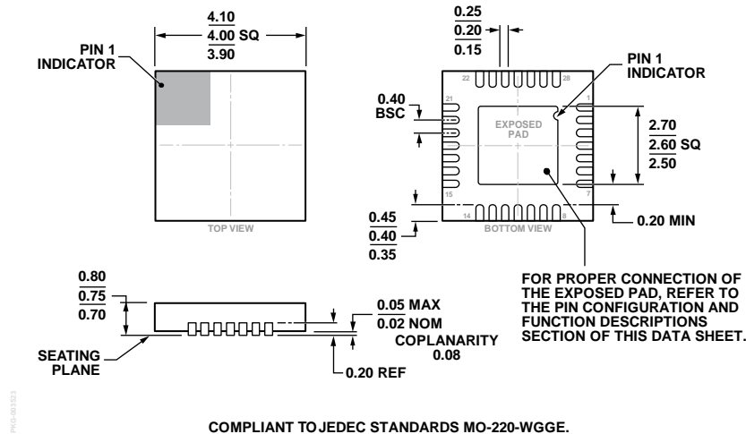
Figure 31. 28-Lead Lead Frame Chip Scale Package [LFCSP_WQ] 4 mm x 4 mm Body, Very Very Thin Quad (CP-28-5) Dimensions shown in millimeters
