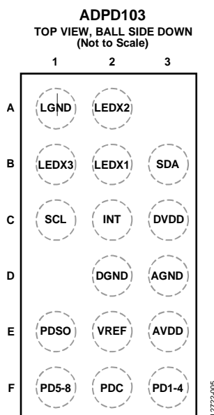
Figure 5. 16-Ball WLCSP Pin Configuration
