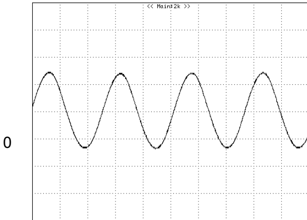
Figure 11: Input Terminal Ripple Current, i_c , at full rated output current and nominal input voltage with 12\mu\text{H} source impedance and 33\mu\text{F} electrolytic capacitor ( 100\text{mA}/\text{div} , 1\mu\text{s}/\text{div} )
