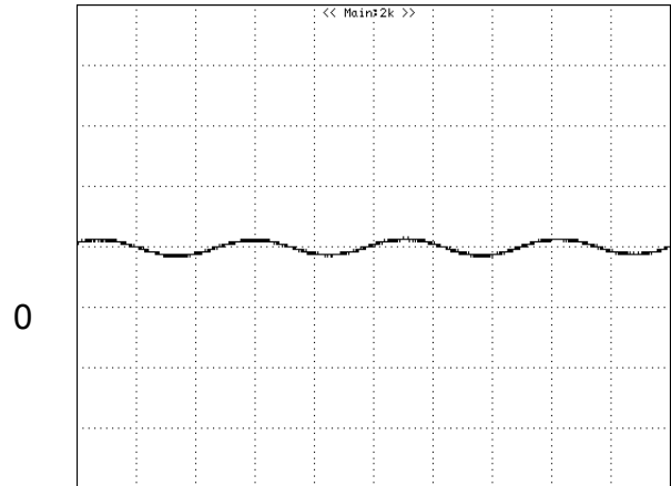
Figure 12: Input reflected ripple current, i_s , through a 12\mu\text{H} source inductor at nominal input voltage and rated load current ( 20\text{mA}/\text{div} , 1\mu\text{s}/\text{div} )
