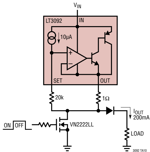
Pulsed Current Source, Load to Ground
