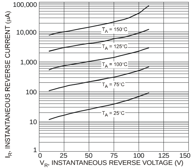
Fig. 4 Typical Reverse Characteristics, B350A thru B360A
