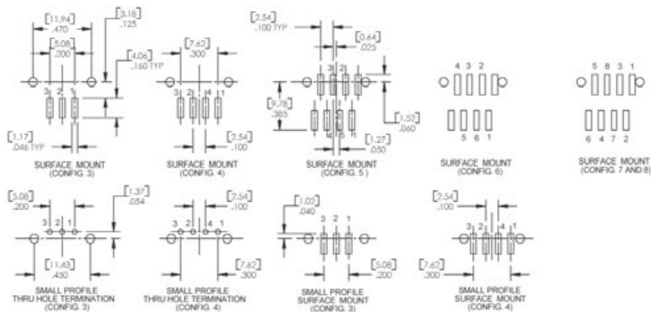
RECOMMENDED PC BOARD LAYOUTS
