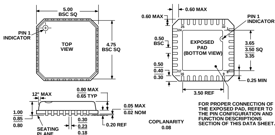
Figure 55. 32-Lead Lead Frame Chip Scale Package [LFCSP_VQ] 5 mm x 5 mm Body, Very Thin Quad (CP-32-4) Dimensions shown in millimeters
