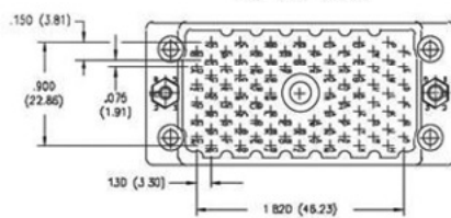
90 PIN PLUG
