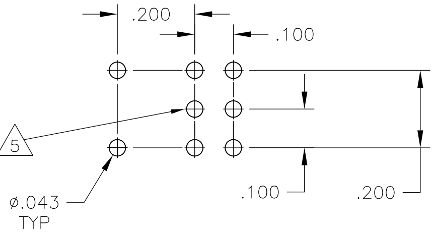
PCB HOLE LAYOUT
