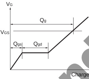
Fig.13 Gate Charge Waveform
