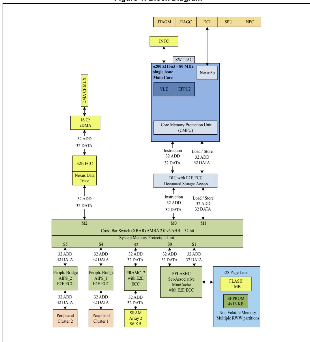
Figure 1. Block Diagram
