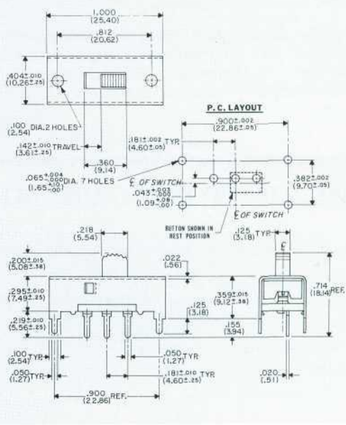
GP-132 Single Pole Double Throw (spring return)
