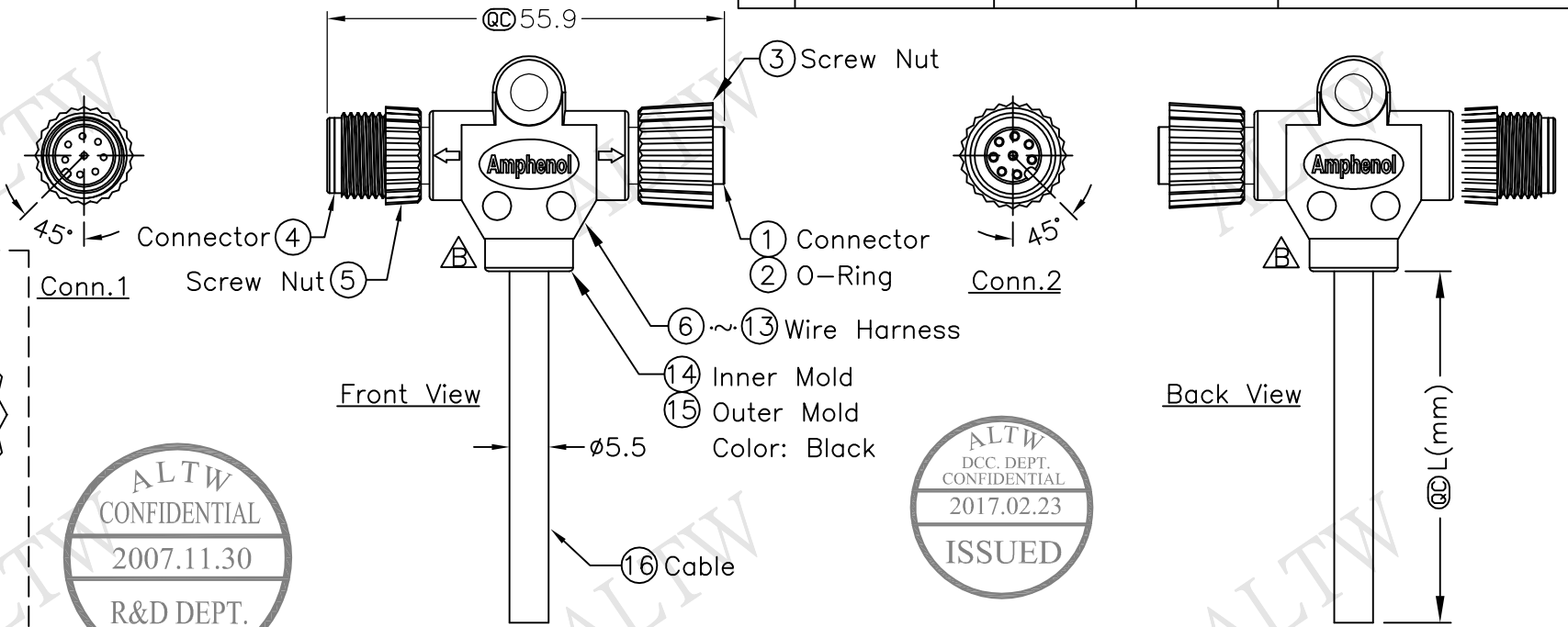
Conn.1 Pin Assignments Front View
