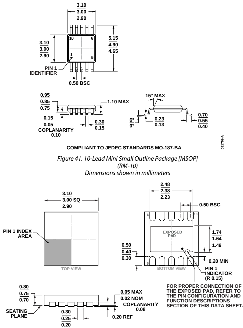
Figure 42. 10-Lead Lead Frame Chip Scale Package [LFCSP_WD] 3 mm × 3 mm Body, Very Very Thin, Dual Lead (CP-10-9) Dimensions shown in millimeters
