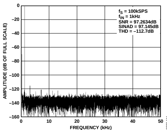
Figure 11. AD7989-1 FFT Plot
