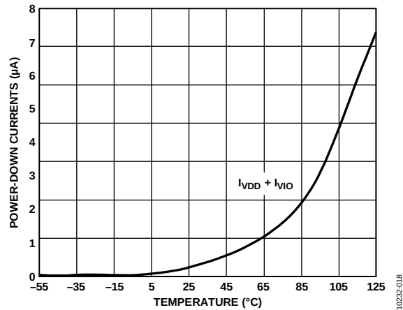
Figure 22. Power-Down Currents vs. Temperature
