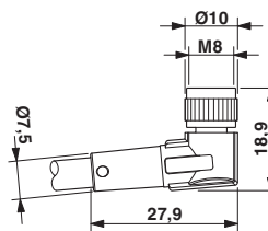
Dimensioned drawing
