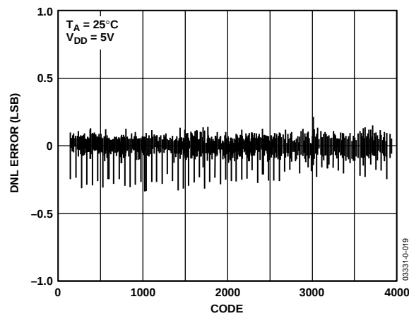
Figure 19. AD5348 Typical DNL Plot
