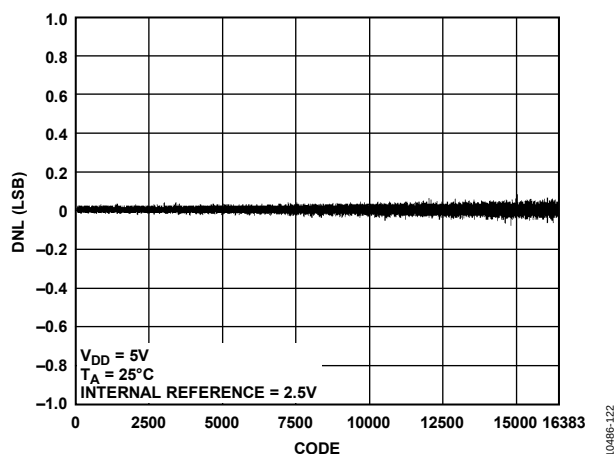
Figure 16. AD5695R DNL
