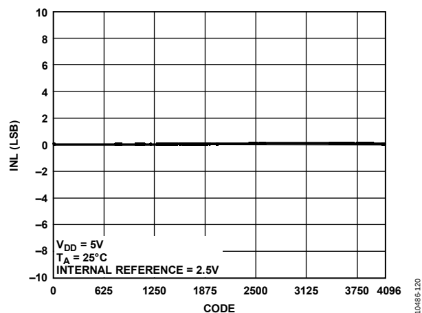
Figure 14. AD5694R INL
