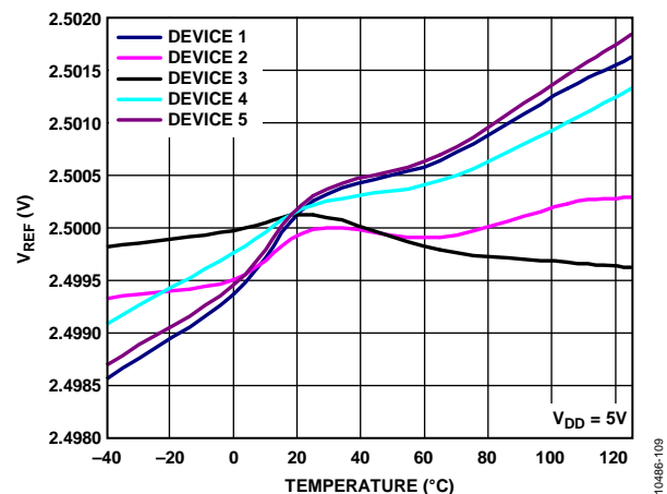
Figure 6. Internal Reference Voltage vs. Temperature (Grade A)
