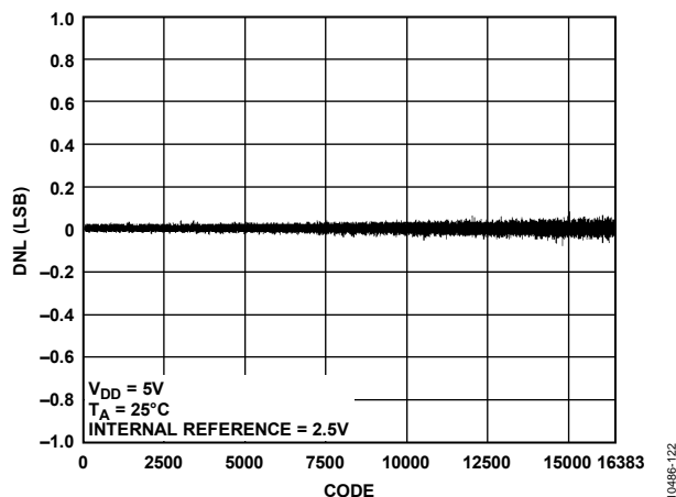
Figure 16. AD5695R DNL
