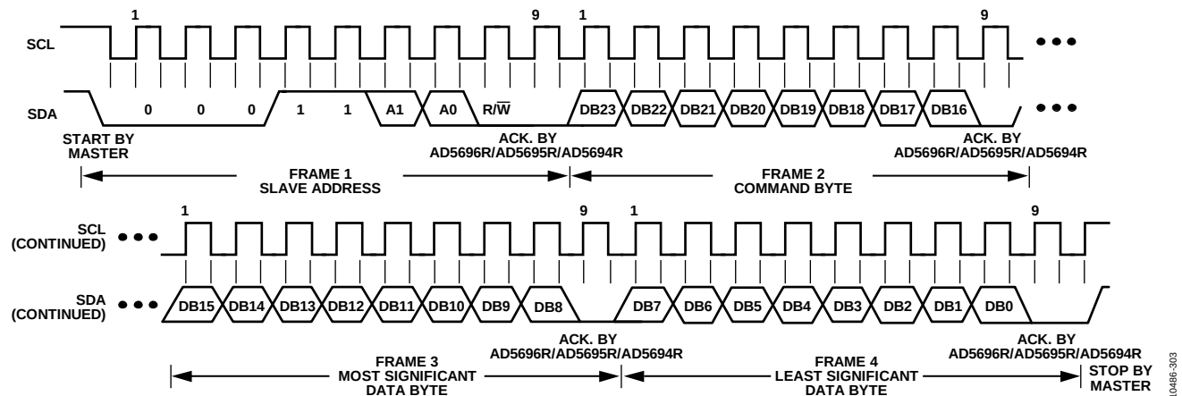
Figure 50. I²C Write Operation
