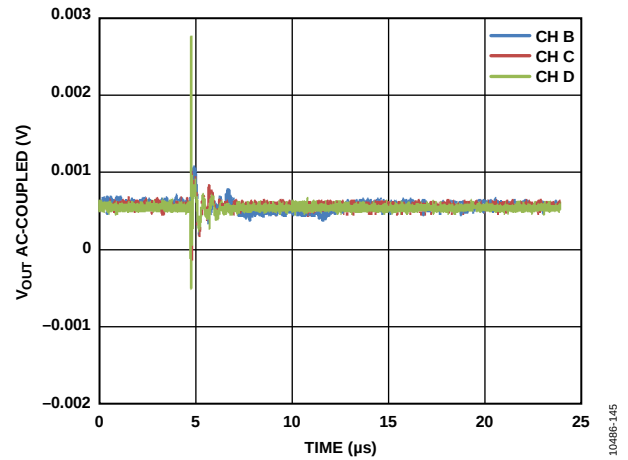
Figure 38. Analog Crosstalk, Channel A
