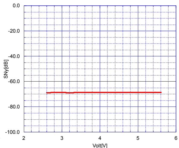
S/N Ratio vs. Operating Voltage ( Y_{signal} , T_a = 25^\circ\text{C} )
