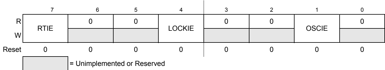
Figure 7-9. S12CPMU_UHV_V6 Interrupt Enable Register (CPMUINT)
