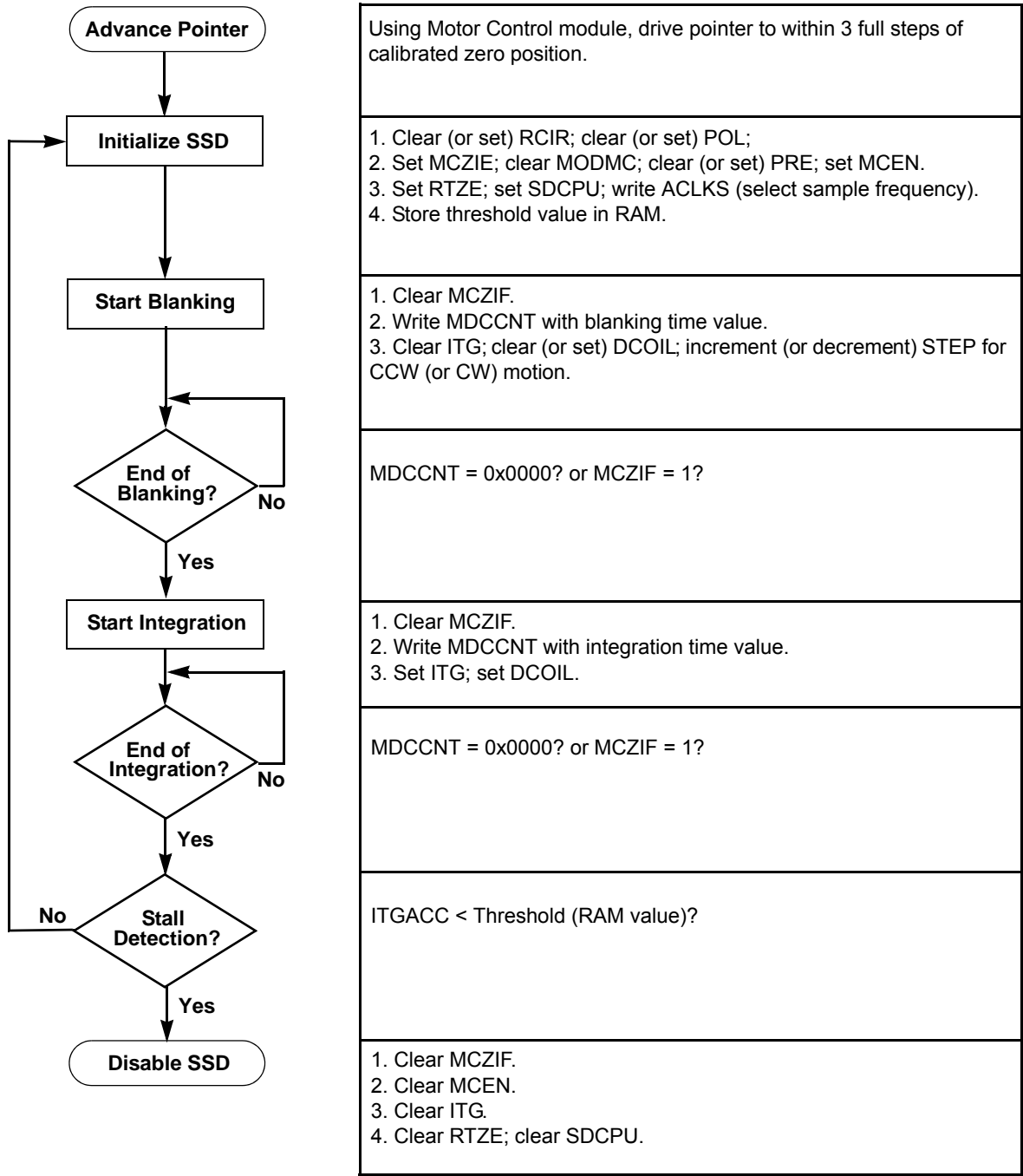
Figure 17-15. Return-to-Zero Flowchart
