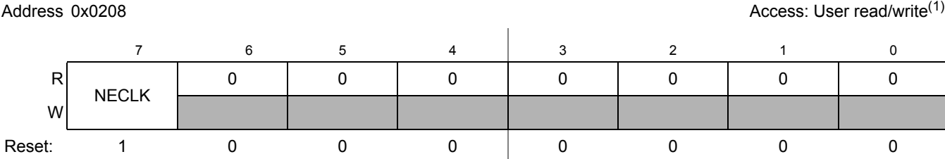
Figure 2-5. ECLK Control Register (ECLKCTL)
