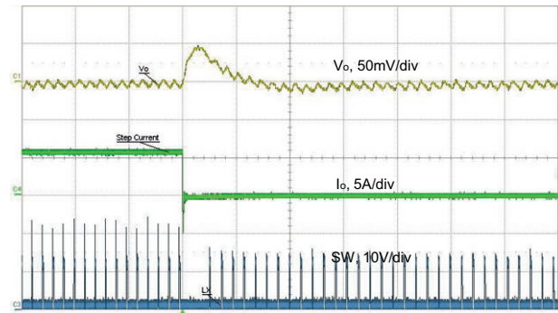
Fig. 54 - Load Release, 6 A to 0.1 A, 1 A/ \mu\text{s} , t = 10\text{ }\mu\text{s/div} Forced Continuous Conduction Mode
