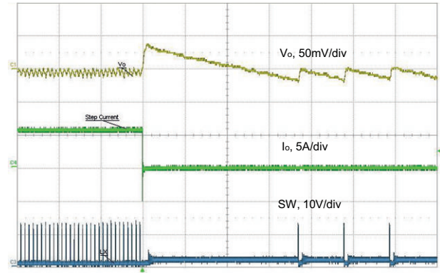
Fig. 53 - Load Release, 6 A to 0.1 A, 1 A/ \mu\text{s} , t = 20\text{ }\mu\text{s/div} Skip Mode Enabled
