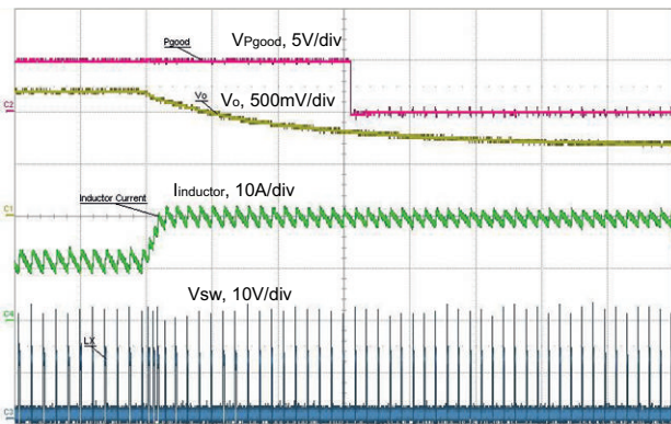
Fig. 57 - Overcurrent Protection Behavior, t = 10\text{ }\mu\text{s/div}
