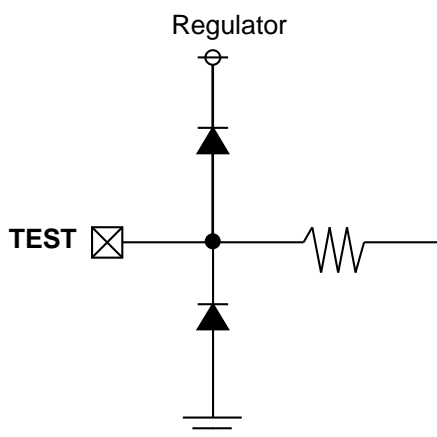
&lt;TEST pin&gt;
