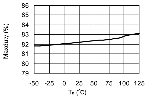
R1245x00xG/R1245x00xH (V IN =12V)
