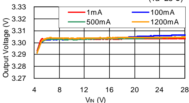
R1245x00xE/R1245x00xF V OUT =3.3V
