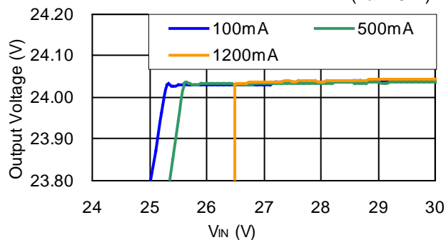
R1245x00xC/R1245x00xD V OUT =24V
