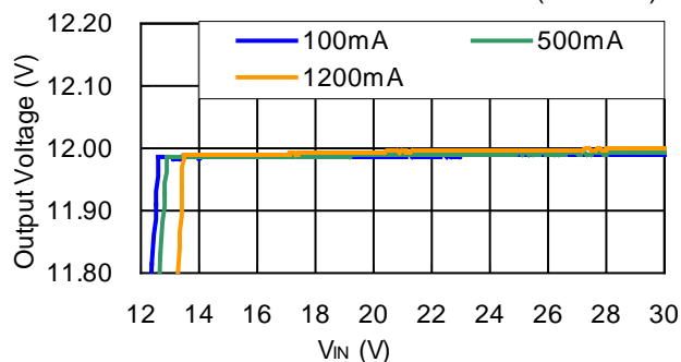
R1245x00xC/R1245x00xD V OUT =12V
