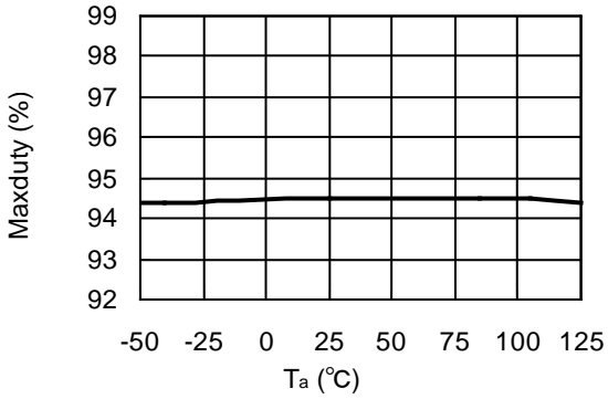
R1245x00xA/R1245x00xB ( V_{IN}=12V )
