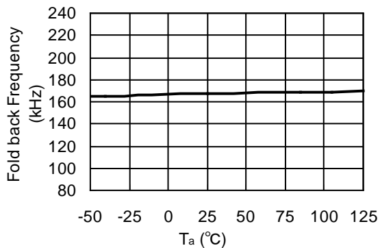
R1245x00xB ( V_{IN}=12V )
