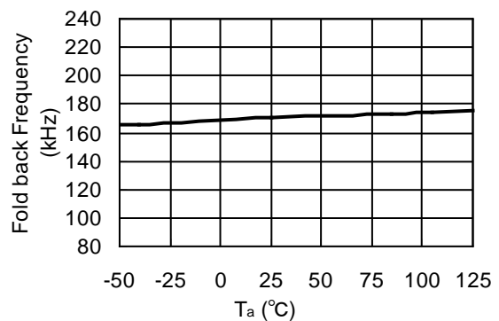
R1245x00xD ( V_{IN}=12V )
