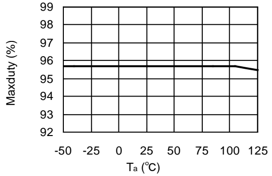
R1245x00xC/R1245x00xD ( V_{IN}=12V )
