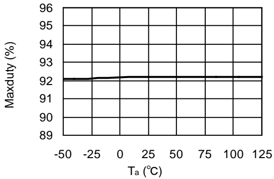
R1245x00xE/R1245x00xF ( V_{IN}=12V )
