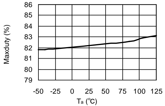
R1245x00xG/R1245x00xH ( V_{IN}=12V )
