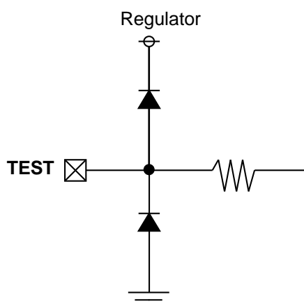
&lt;TEST pin&gt;
