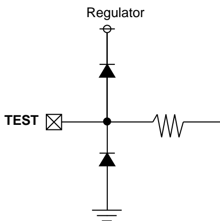
<TEST pin>
