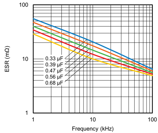
ESR as a function of frequency (2000 V DC ) (typical curve)
