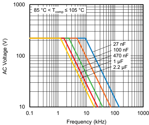
Maximum RMS voltage as a function of frequency (630 V DC )
