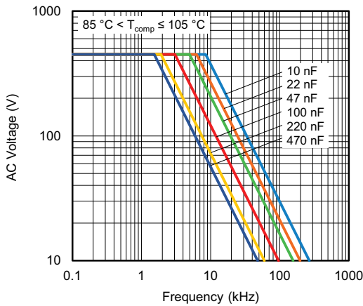
Maximum RMS voltage as a function of frequency (1250 V DC )
