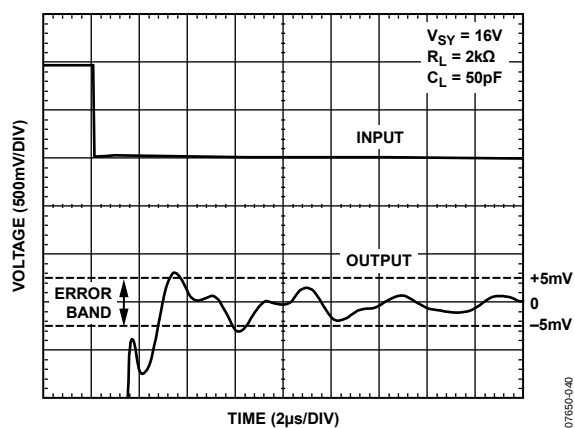
Figure 43. Negative Settling Time to 0.1%
