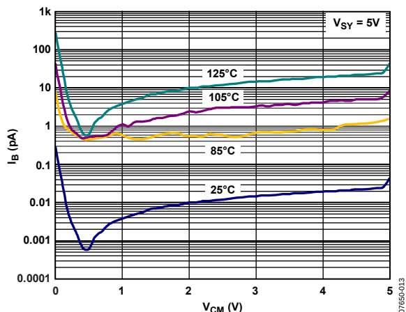
Figure 10. Input Bias Current vs. Input Common-Mode Voltage
