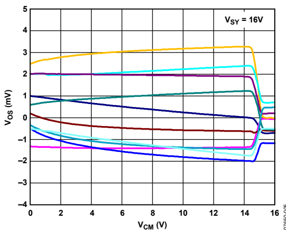
Figure 8. Input Offset Voltage vs. Common-Mode Voltage
