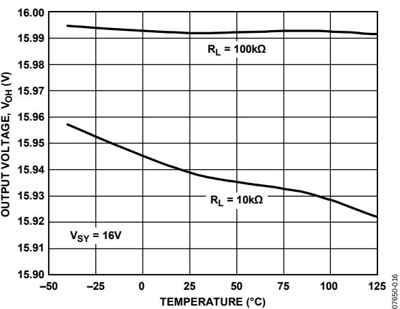
Figure 19. Output Voltage ( V_{OH} ) vs. Temperature
