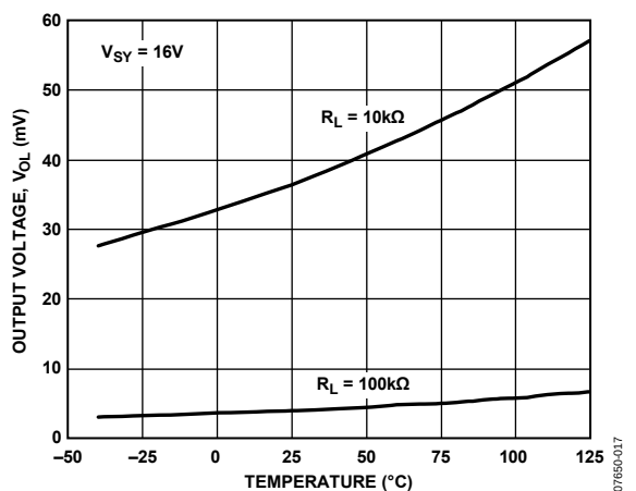
Figure 20. Output Voltage ( V_{OL} ) vs. Temperature
