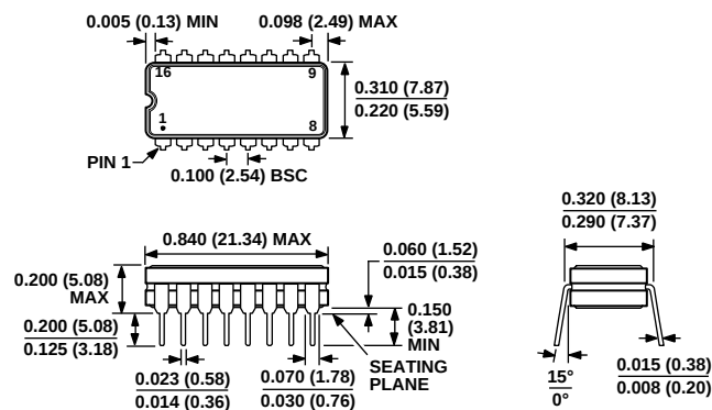
Figure 35. 16-Lead Ceramic Dual In-Line Package [CERDIP]
