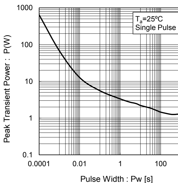
Fig.4 Single Pulse Maxmum Power dissipation
