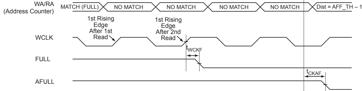
Figure 2-36 • FIFO FULL Flag and AFULL Flag Deassertion
