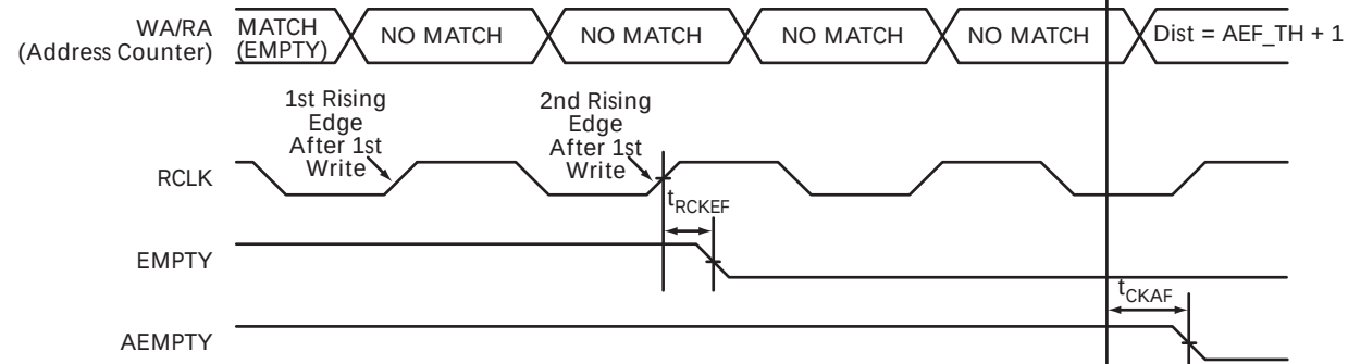
Figure 2-35 • FIFO EMPTY Flag and AEMPTY Flag Deassertion
