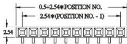
(TYPE A)
