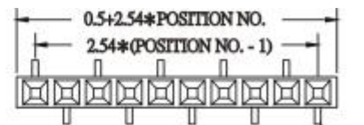
(TYPE B1)
