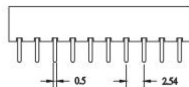
(TYPE B2)
