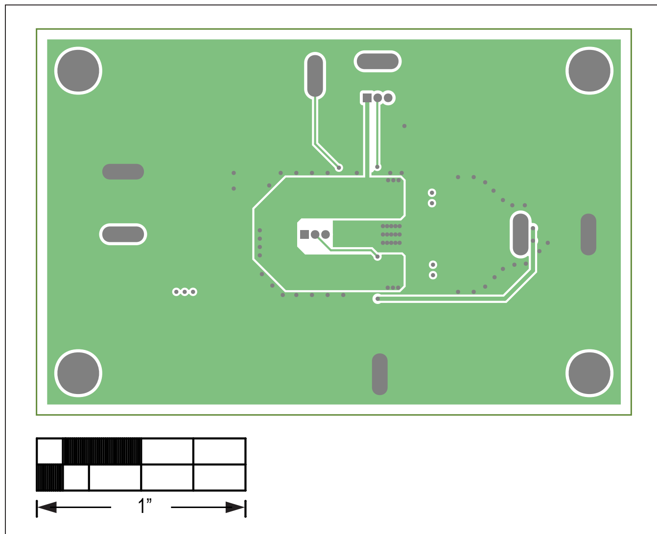
MAX17633B EV Kit — Layer3 GND
