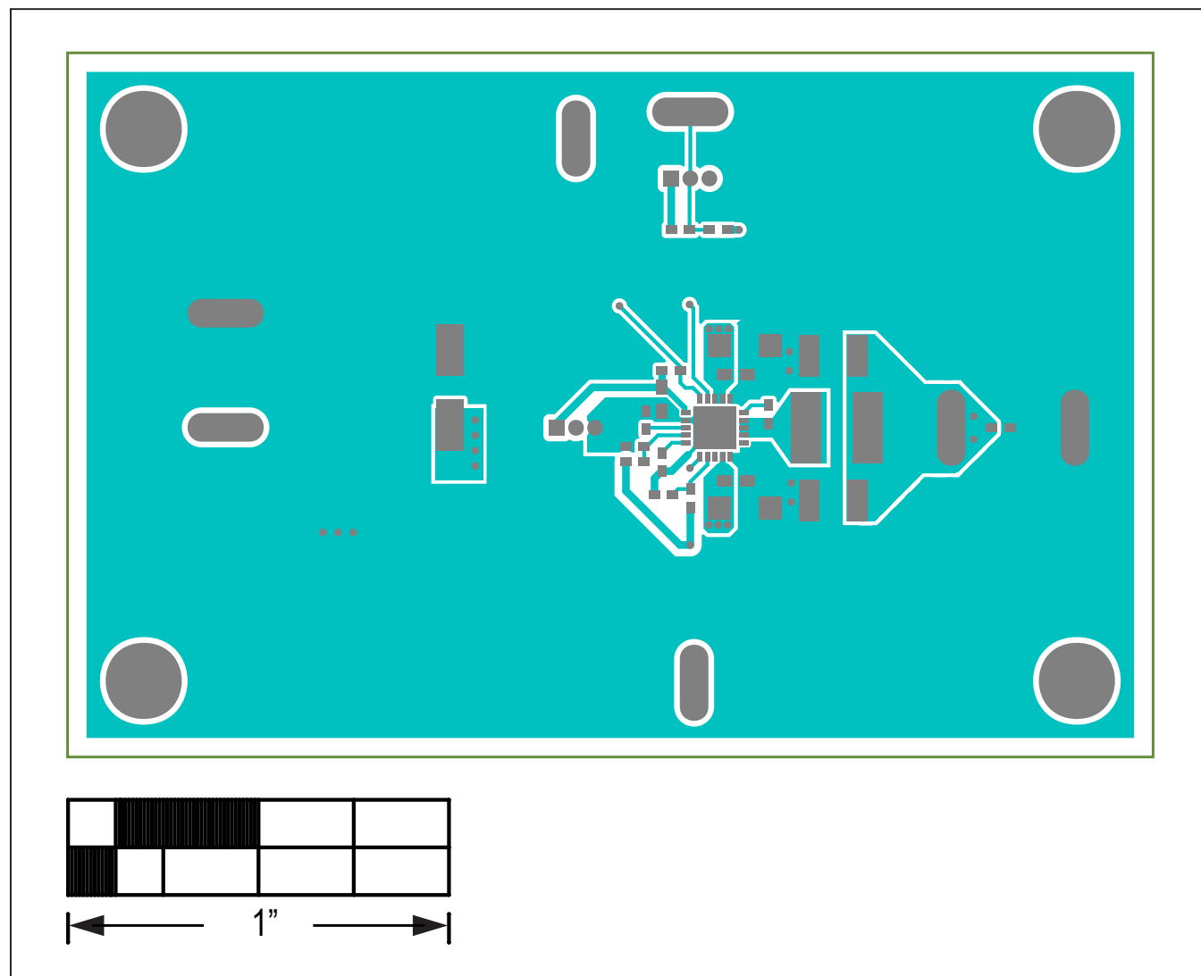
MAX17633B EV Kit — Top
