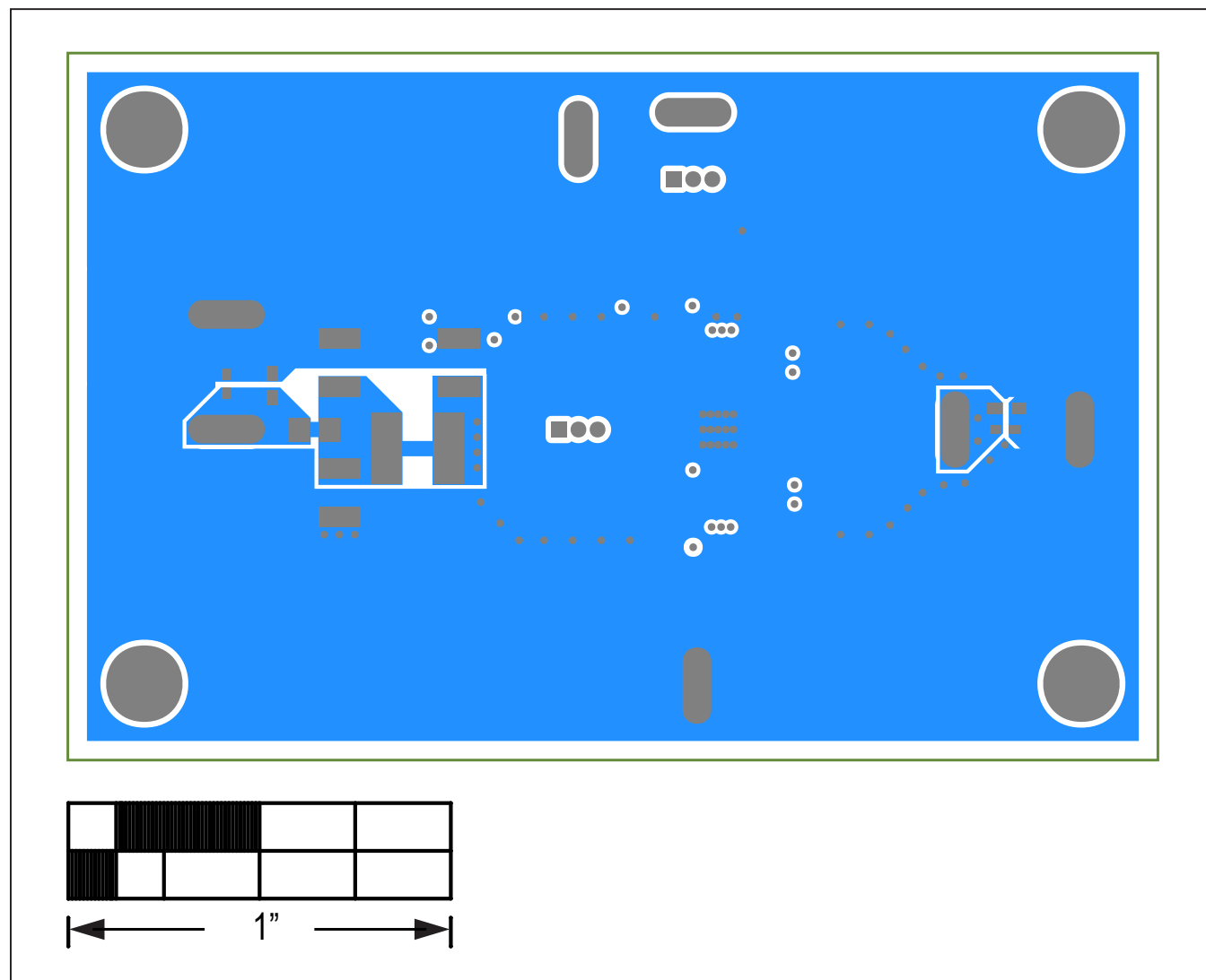
MAX17633B EV Kit — Bottom
