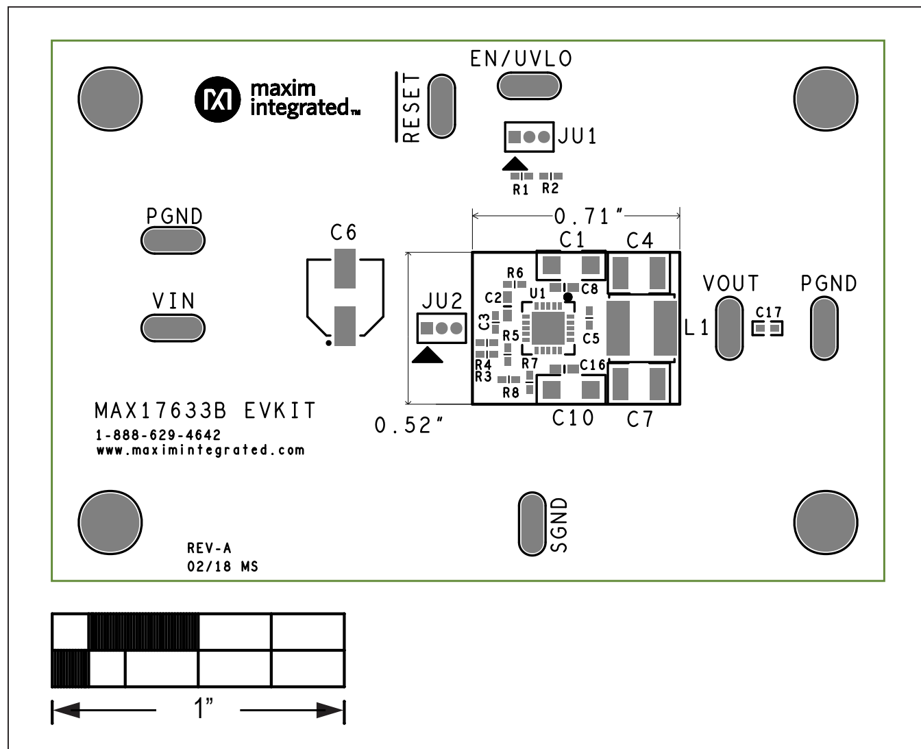
MAX17633B EV Kit — Top Silkscreen
