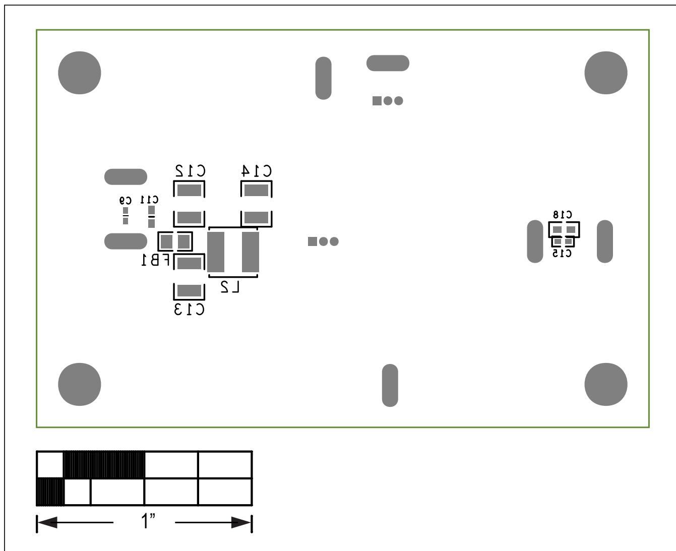
MAX17633B EV Kit — Bottom Silkscreen
