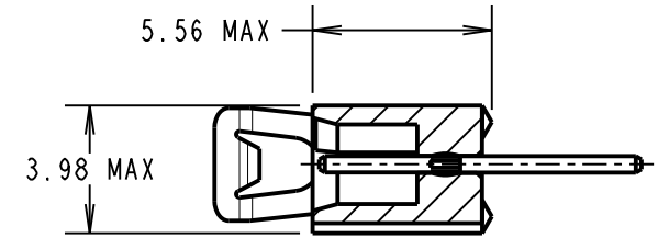
SECTION X-X
