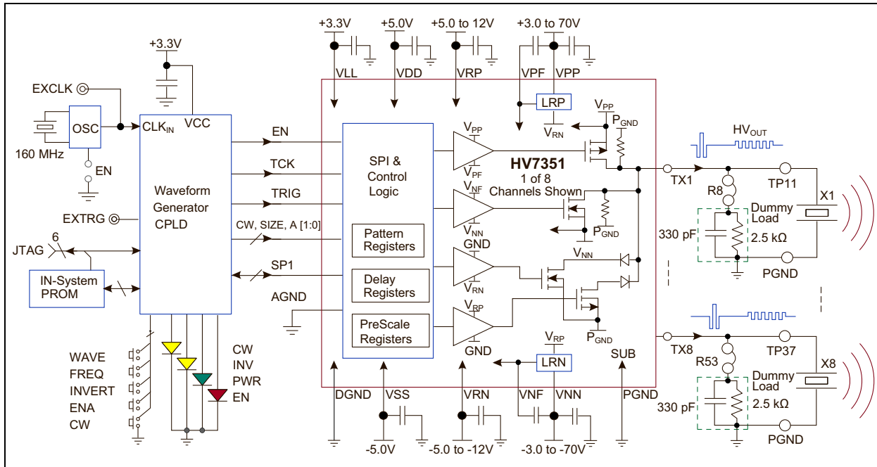
FIGURE 1-1: Block Diagram.
