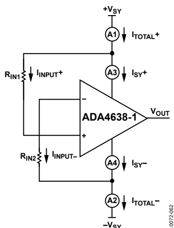
Figure 62. Comparator B
